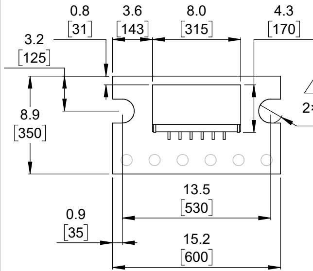
① Board dimensions (top view) Scale 3:1
