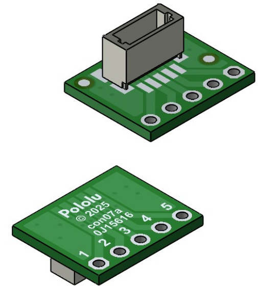
③ Isometric view Scale 3:1
