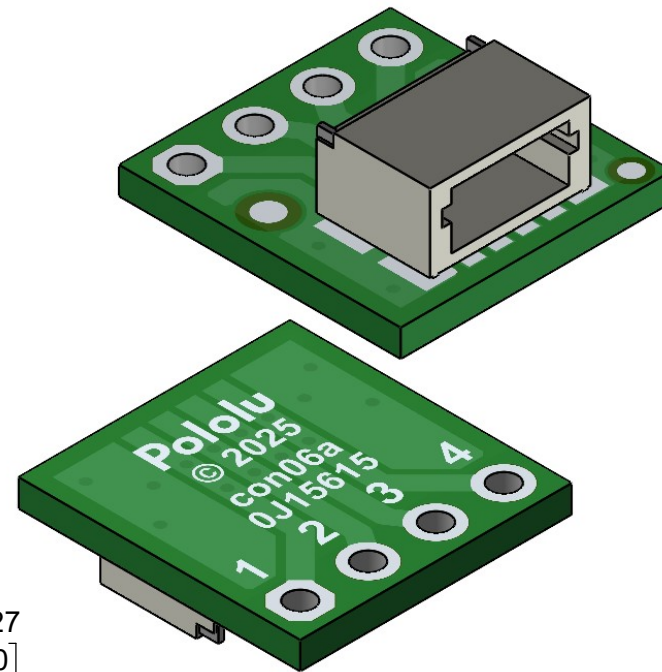
③ Isometric view Scale 5:1
