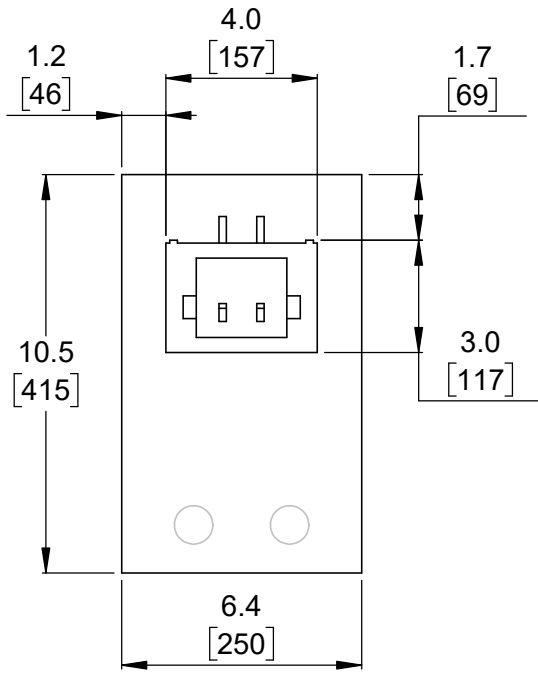
① Board dimensions (top view) Scale 5:1
