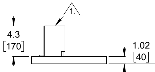
④ Profile Scale 3:1
