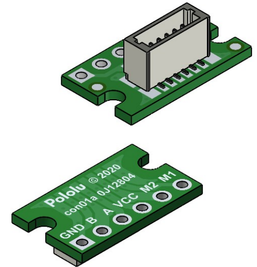
③ Isometric view Scale 3:1
