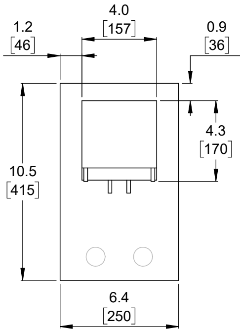
① Board dimensions (top view) Scale 5:1
