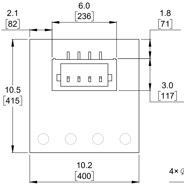
① Board dimensions (top view) Scale 5:1
