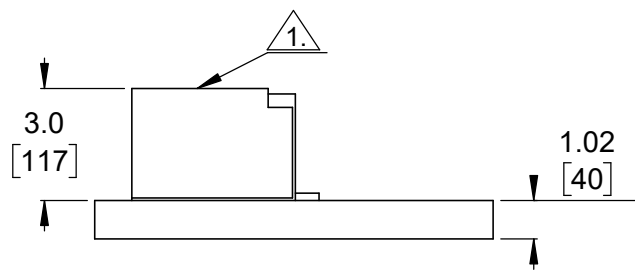
④ Profile Scale 5:1
