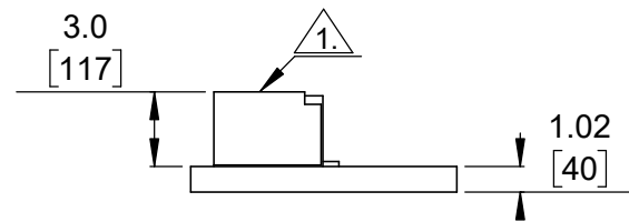
④ Profile Scale 3:1
